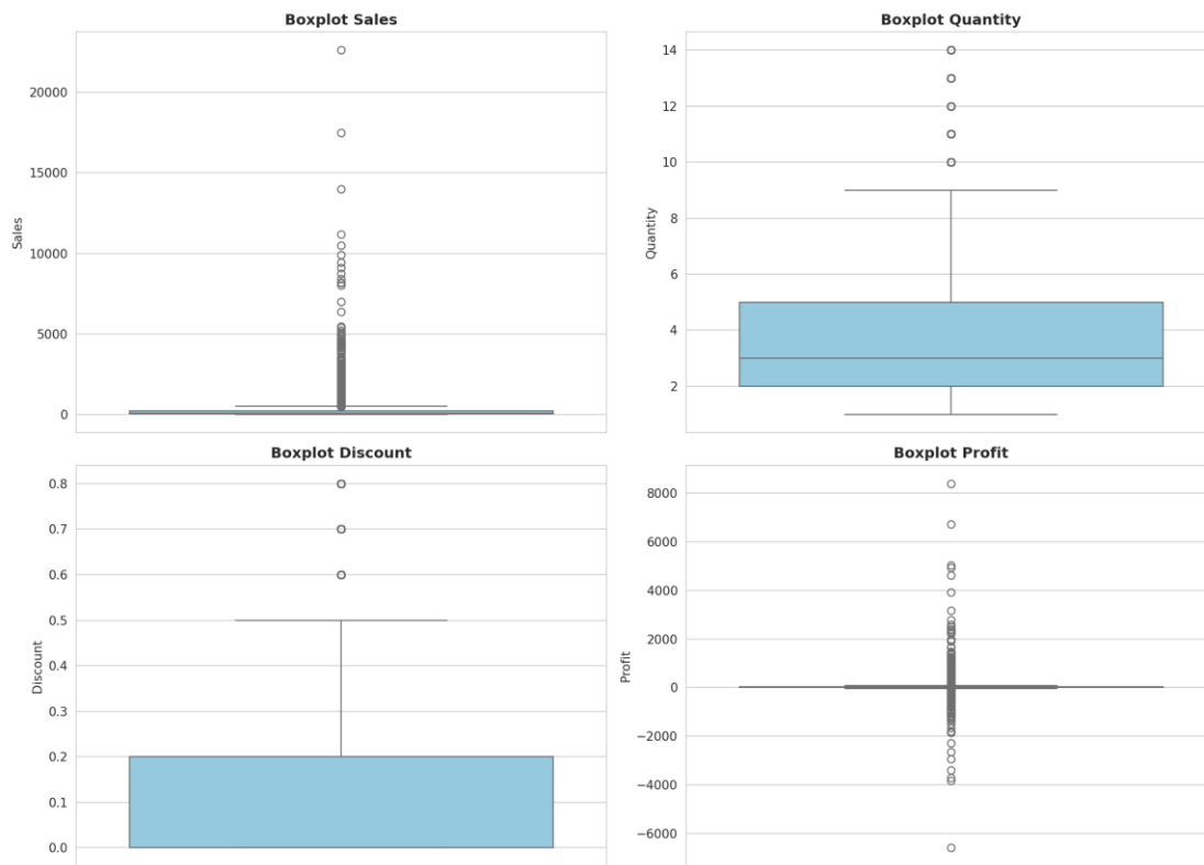
Gambar 2. Boxplot Sales, Quantity, Discount, dan Profit
