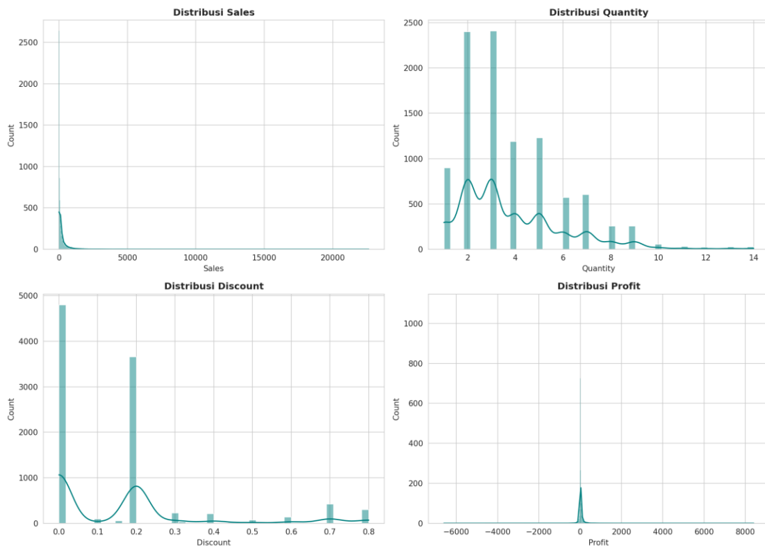
Gambar 1. Distribusi Sales, Quantity, Discount, dan Profit
