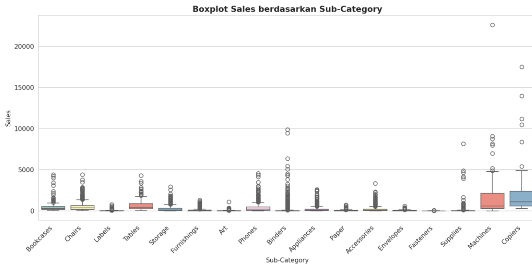
Gambar 4. Boxplot Sales berdasarkan Sub-Category
