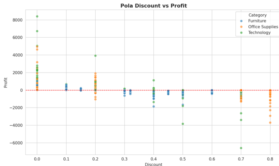
Gambar 5. Discount vs Profit per Category
