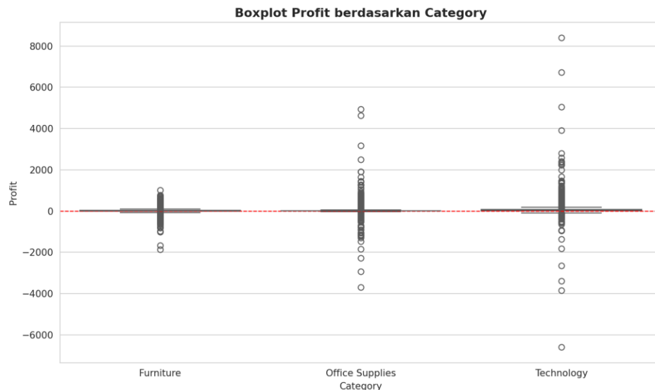
Gambar 3. Boxplot Profit berdasarkan Category
