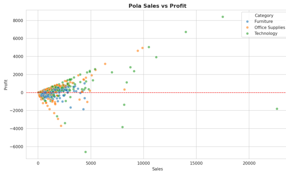
Gambar 6. Sales vs Profit per Category
