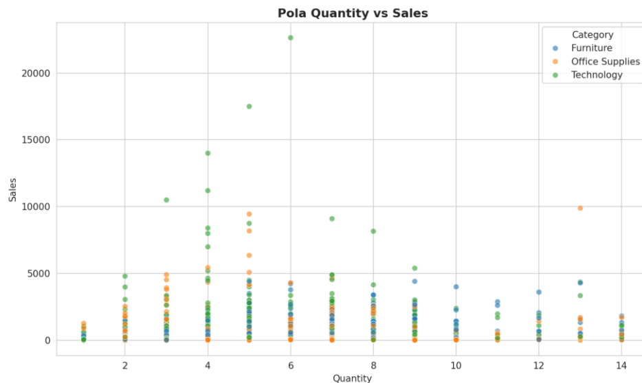
Gambar 7. Quantity vs Sales per Category
